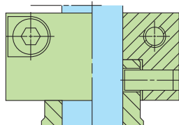
Clamping ring with pin
