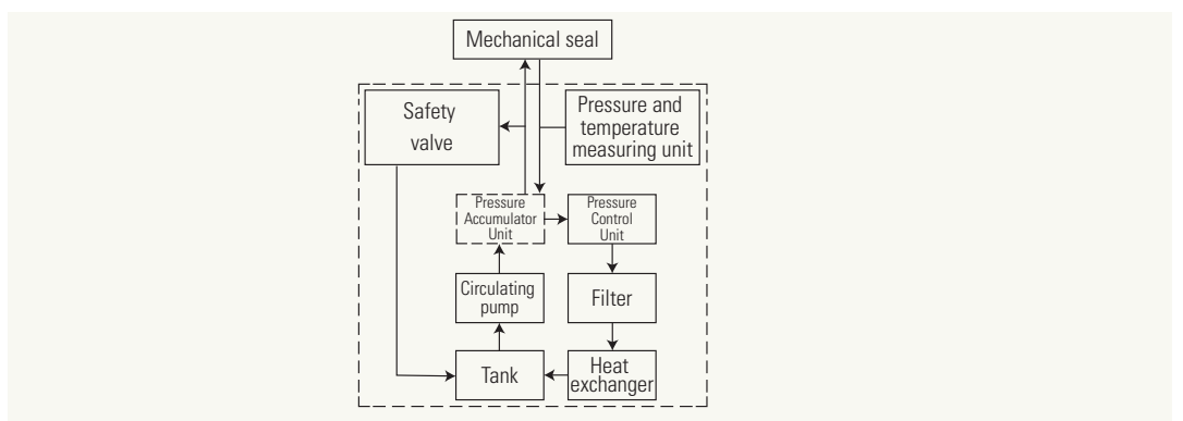
Installation and operating diagram for a BFS system.
